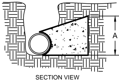
SECTION VIEW
