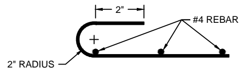
REBAR DETAIL
