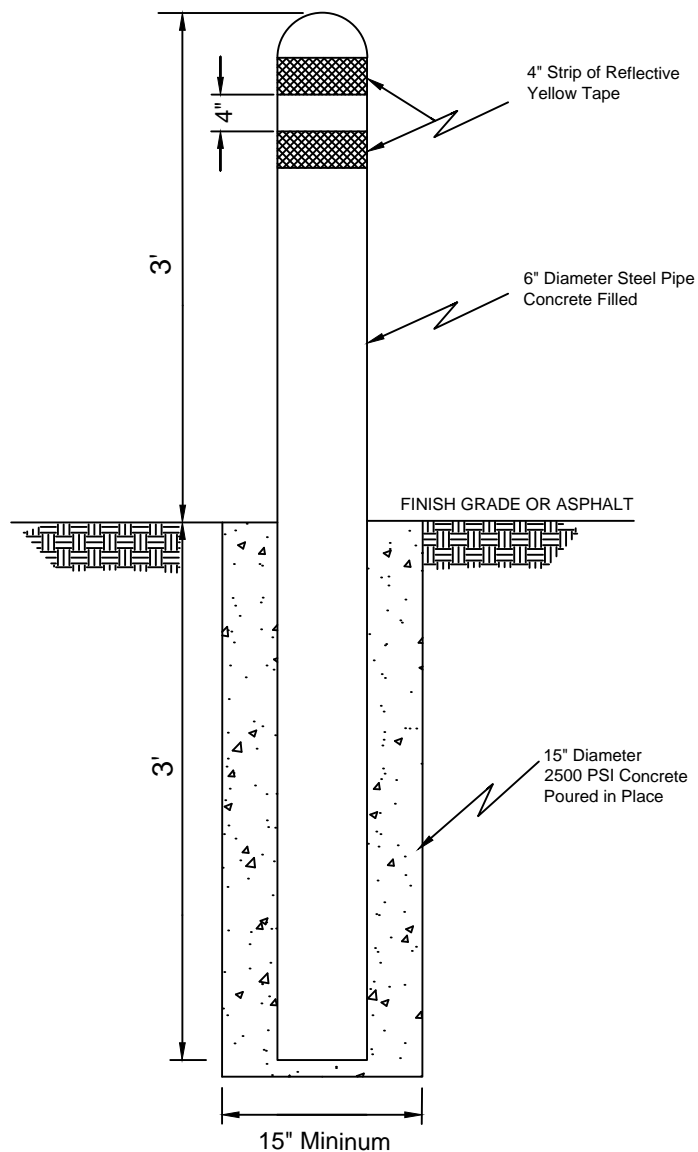
BOLLARD DETAIL
