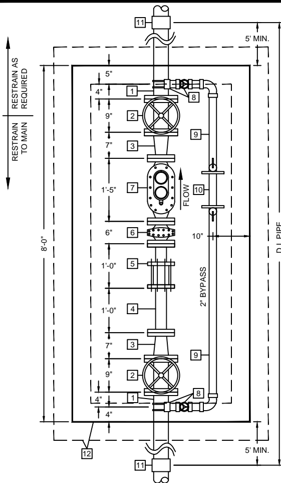
PLAN VIEW
