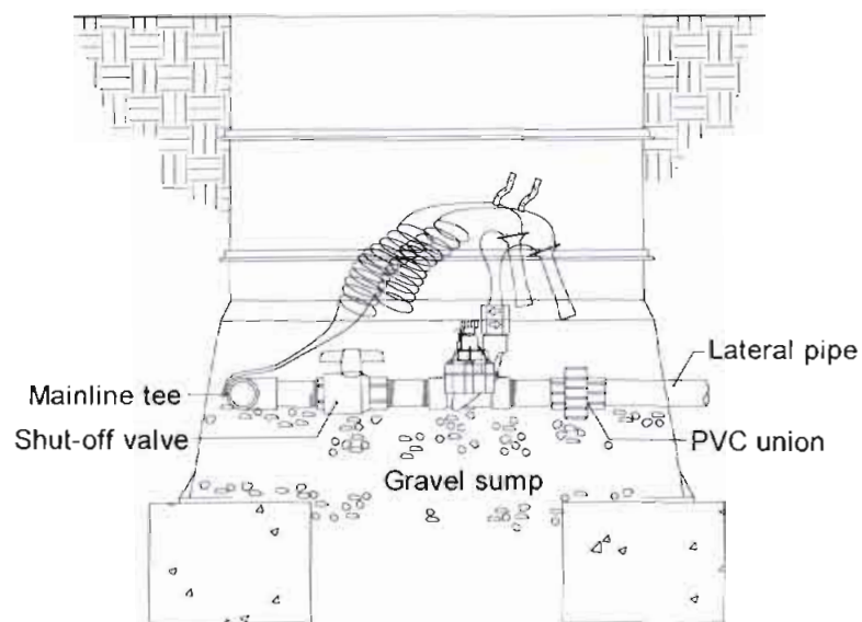
Figure 4-1: Automatic control valve assembly with isolation valve and union
