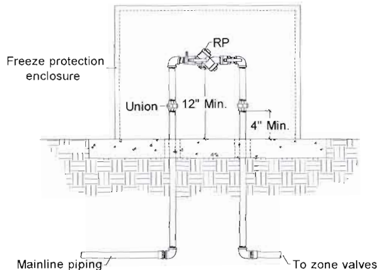
Figure 4-8: RP assembly
