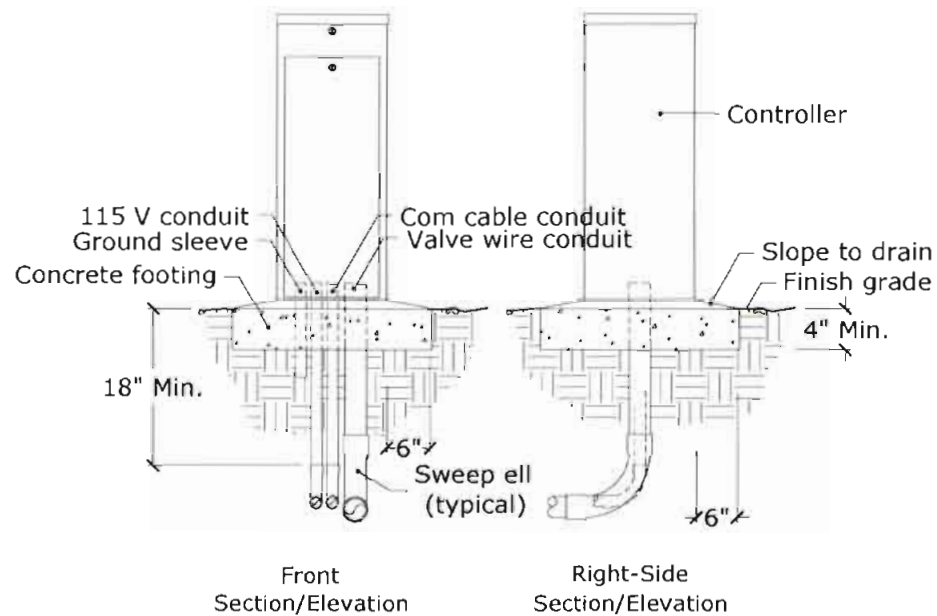
Figure 8-9: Typical pedestal mount controller installation
