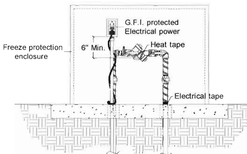
Figure 4-9: Heat tape
