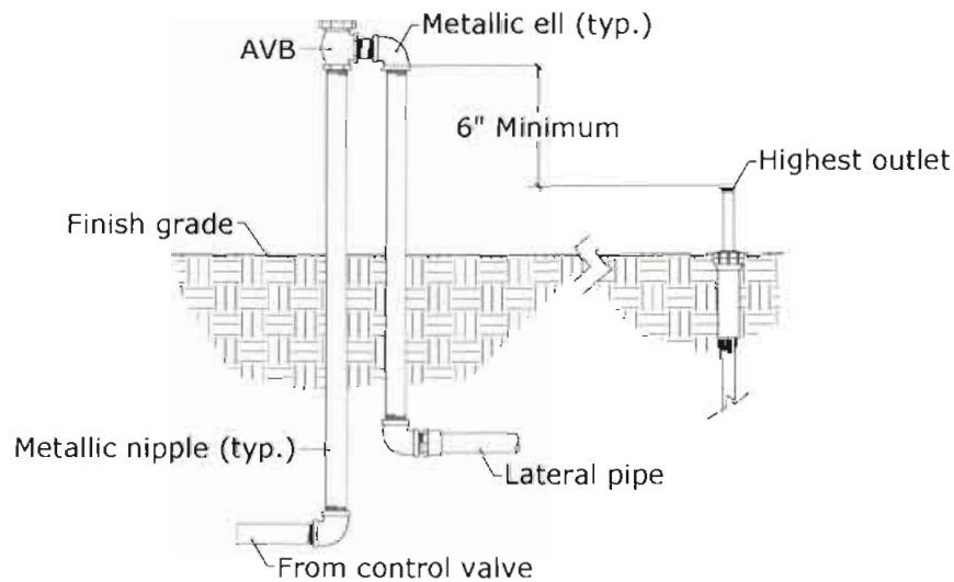
Figure 8-1: AVB assembly
