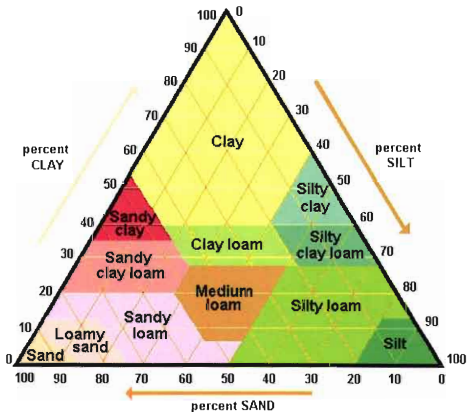
Figure 6-1: Soil Triangle
